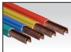
GI & Copper Bolt Type DSL Busbar
