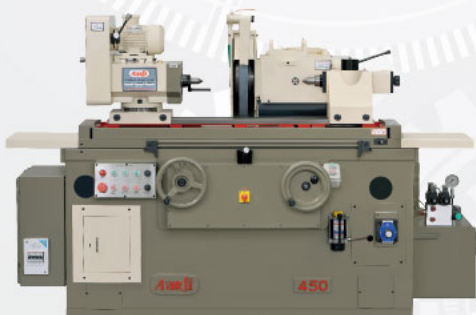
Hydraulic Cylindrical Grinding Machine Size : 450mm to 1500mm
