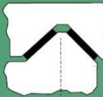
Semi-enclosed Slideway Linear bearing material
