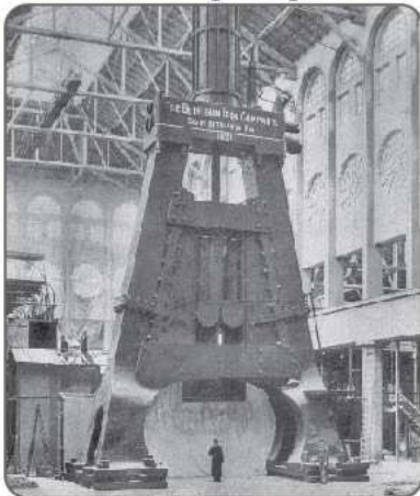
The Great Steam Hammer, 1891, South Bethlehem, Pennsylvania, USA
